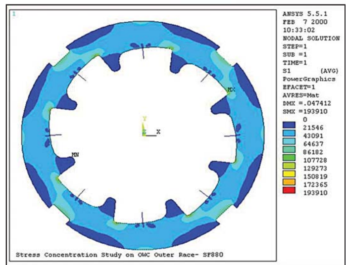
FEA for optimization of component stress
